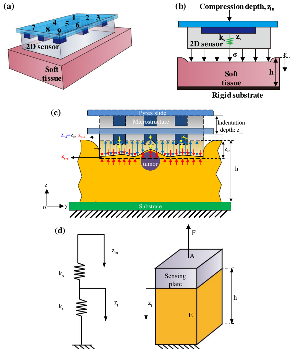
Figure 3.1 Rationale for the Stepwise Compression-Relaxation testing method (a) the whole configuration: the sensor with a 3 \times 3 sensing-plate/transducer array compressing a soft tissue, (b) sensor-tissue interaction of one sensing-plate and the tissue segment underneath, (c) mechanical characterization of a tissue with embedded tumor using the 2D sensor, and (d) Theoretical models of a sensing-plate and the tissue segment underneath: lumped-model with two springs in series and block model with the tissue segment subjected to a deflection input, z_t , from the sensing-plate (out of proportion for better illustration).
