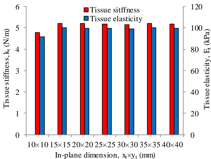
Figure 3.7 FE analysis results of tissue stiffness and estimated tissue elasticity as a function of the tissue in-plane dimension, with the tissue elasticity E_i fixed at 100kPa and tissue thickness h fixed at 12mm.
