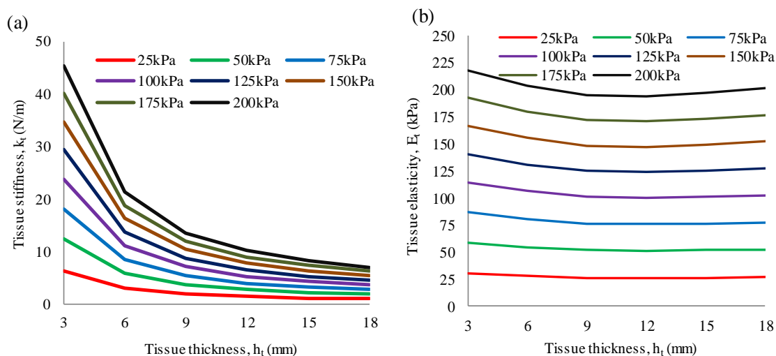
Figure 3.6 FE analysis results of (a) tissue stiffness, and (b) tissue instant elasticity as a function of tissue thickness at different tissue elasticity ( E_i : 25kPa-200kPa), with the tissue in-plane dimension fixed at 20mm×20mm.
